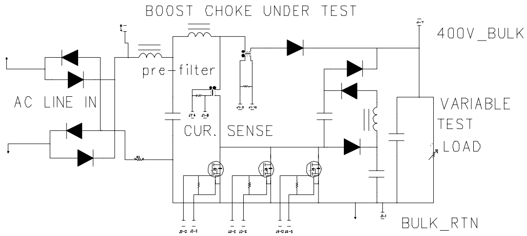
Figure 2. Continuous Conduction Mode PFC Test circuit
