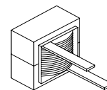
Figure 1. A new type of boost choke construction: gapped ETD ferrite with the new helical wound technology (HWT)
